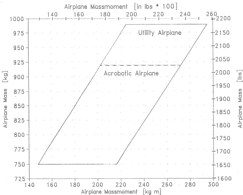
Fig. 6.4 Massmoment Limits
